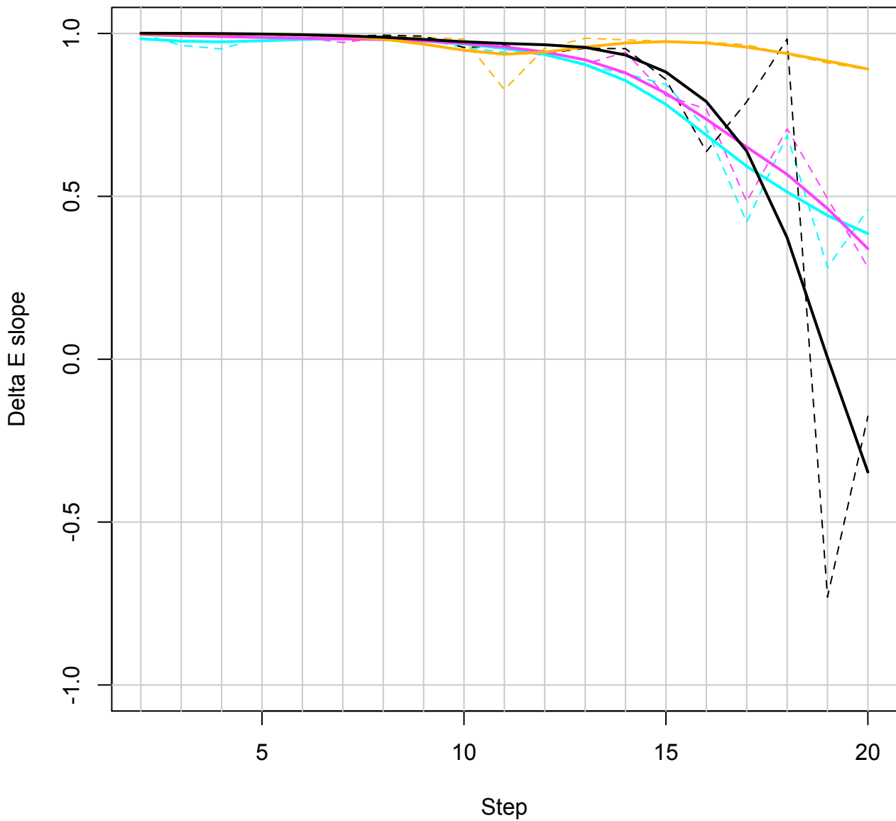
cubic smoothing spline, spar=0.5
