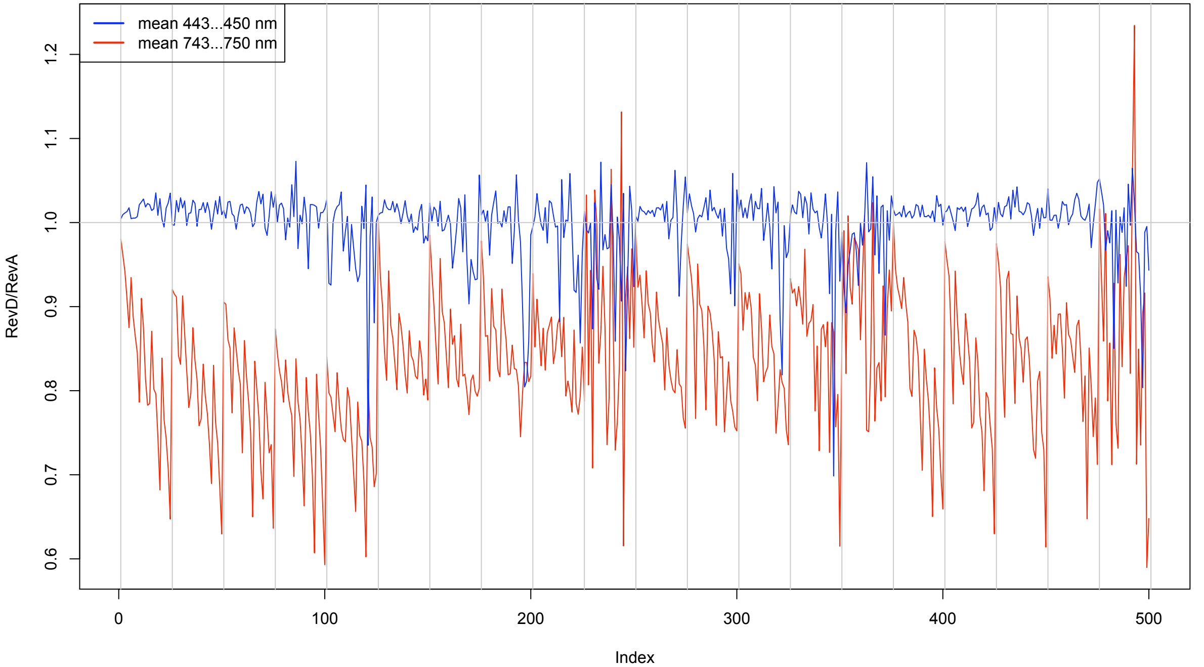
eye-one RevD/RevA, strip length: 25, high res mode, average of 3 bands
